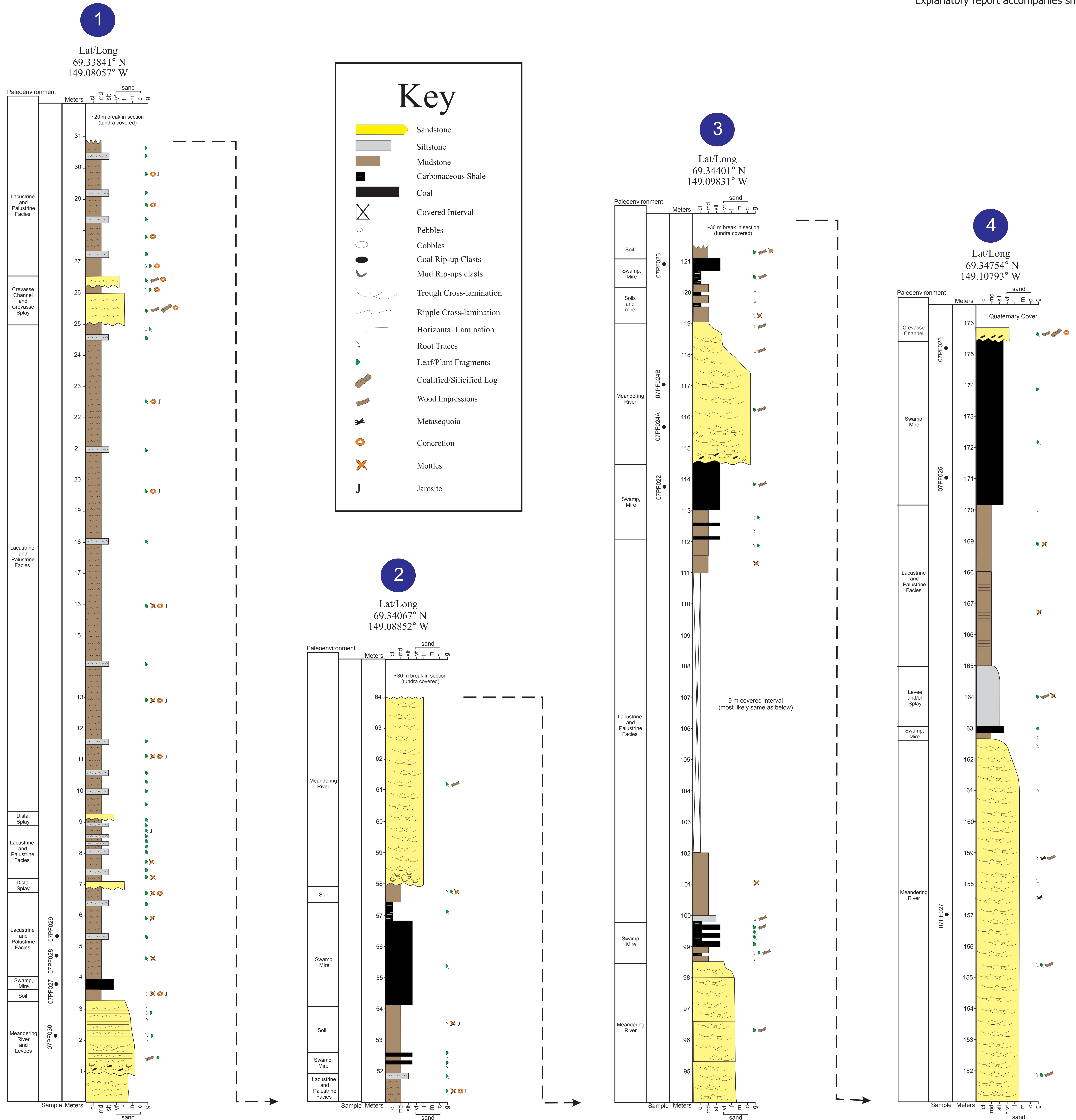
Measured stratigraphic sections of the Prince Creek Formation along the east side of the Toolik River in the Sagavanirktok Quadrangle, Alaska
